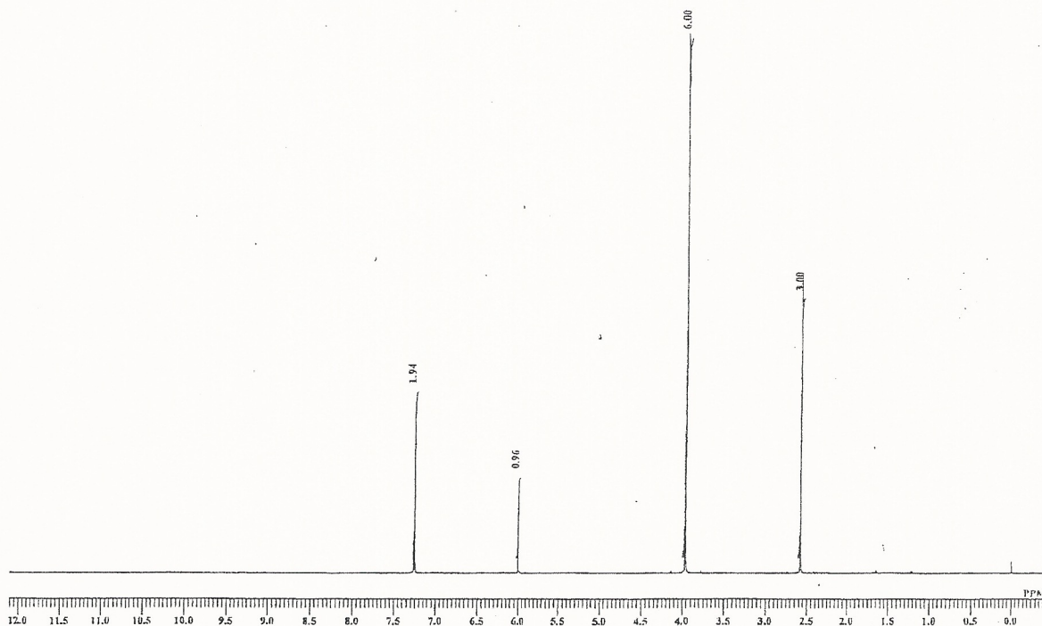
3',5'-Dimethoxy-4'-hydroxy acetophenone (Acetosyringone)
