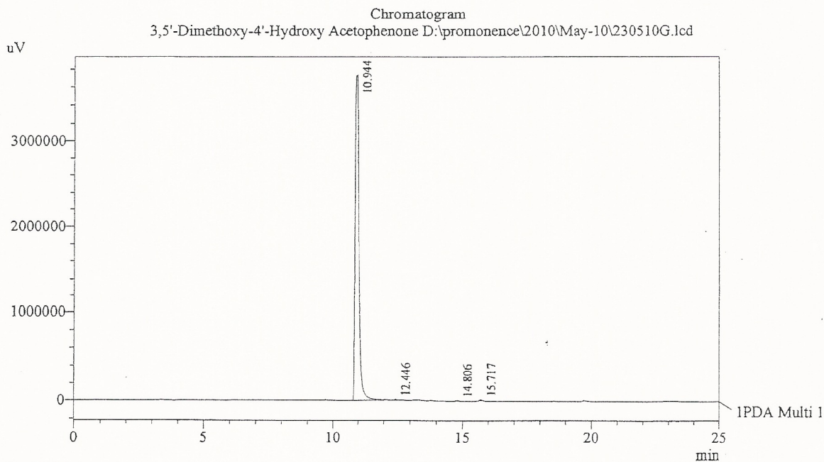
PeakTable PDA Ch1 230nm 4nm
