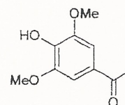
3',5'-Dimethoxy-4'-hydroxy acetophenone (Acetosyringone)
