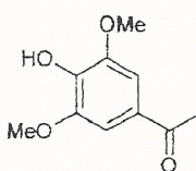
3',5'-Dimethoxy-4'-hydroxy acetophenone (Acetosyringone)
