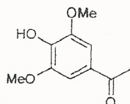
3',5'-Dimethoxy-4'-hydroxy acetophenone (Acetosyringone)
